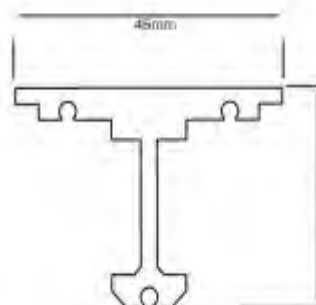
TRACK SECTION
